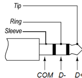
3.5mm TRS Plug
